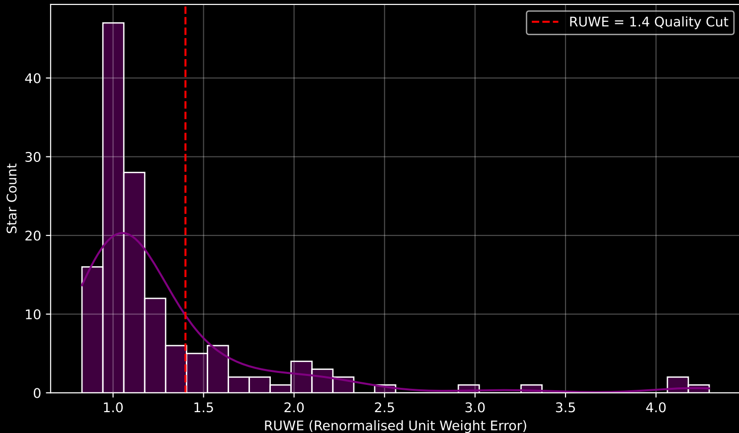
GAPOGEE DR17 Field [044+54_MGA] RUWE Distribution (n= 140)
