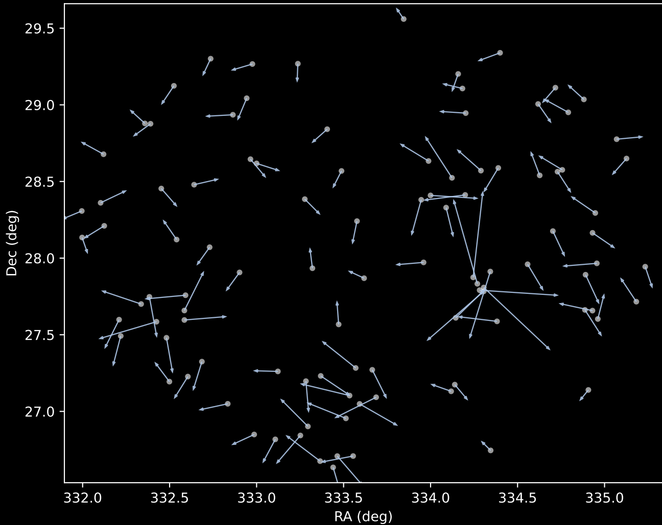
APOGEE DR17 Cluster 1 Proper Motion Vectors (n=103)
