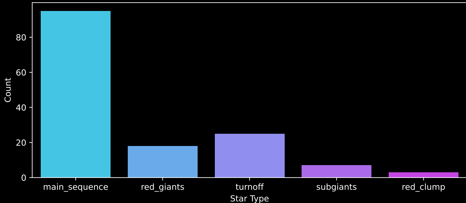
APOGEE DR17 Field: [044+54_MGA] Count plot of Star Type
