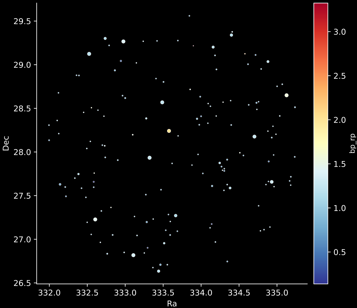
APOGEE DR17 Field: [044+54_MGA] Stars: 148
