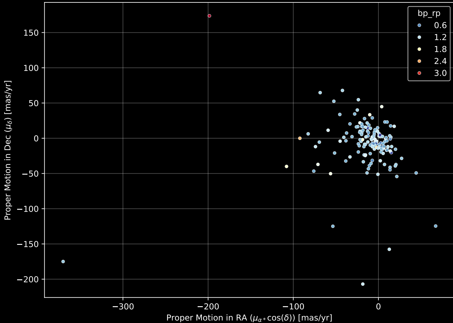
APOGEE DR17 Field: [044+54_MGA] Proper Motion Diagram (n= 148)
