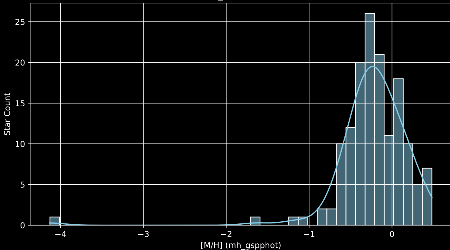
APOGEE DR17 Field: [044+54_MGA [M/H] (mh_gspphot) (n= 148)
