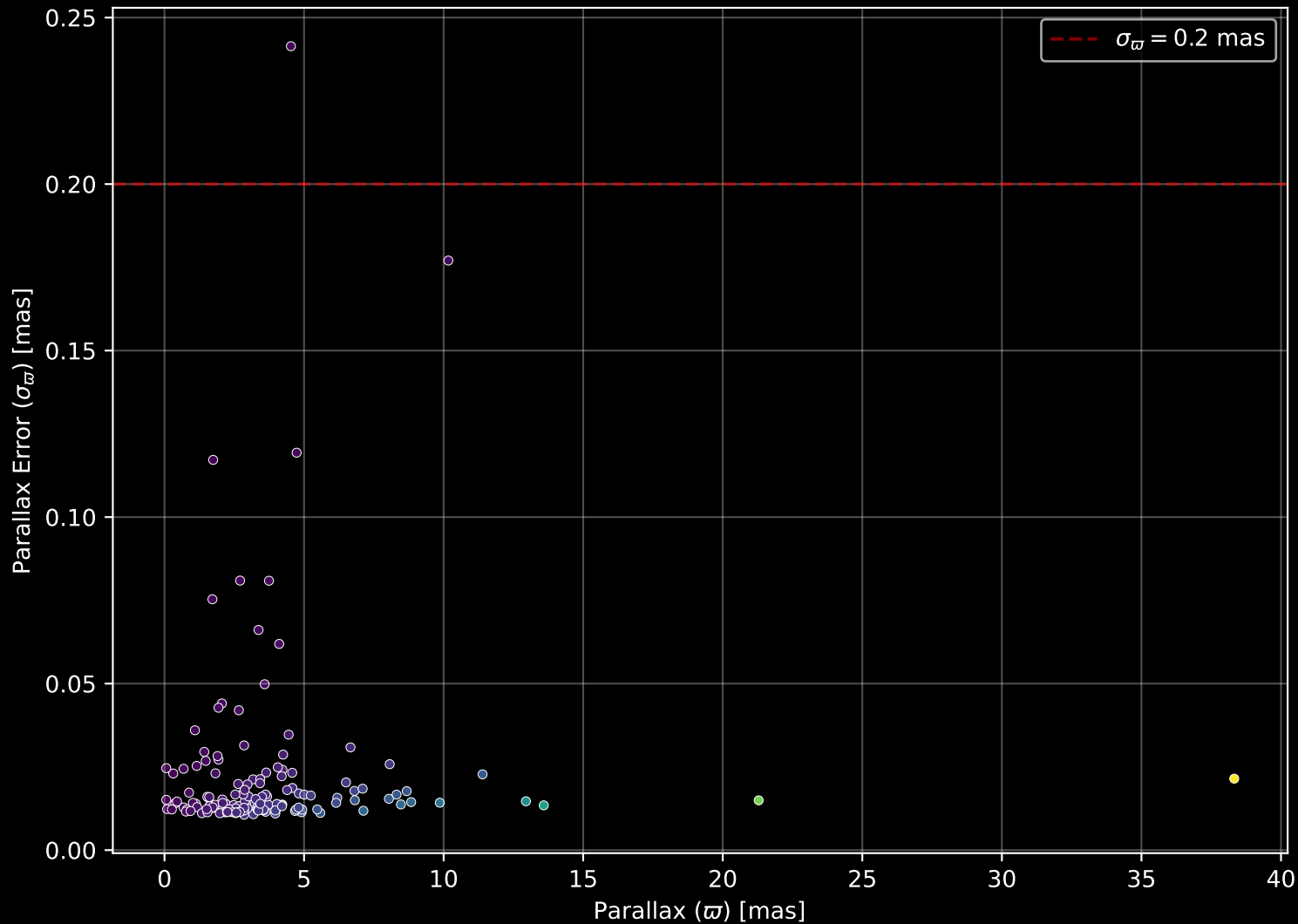
APOGEE DR17 Field: [044+54_MGA] Parallax Quality (n= 148)
